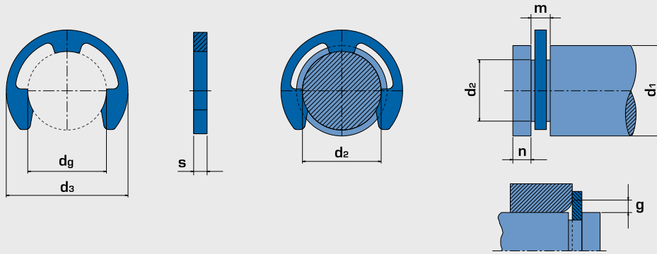
Dimensioni in pollici - Dimensions in inches - Abmessungen in Zoll
